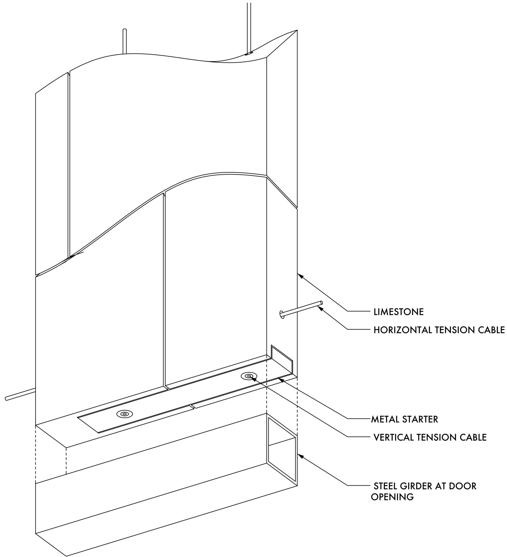
1 Door Girder Detail / Axonometric Detail 1:20
