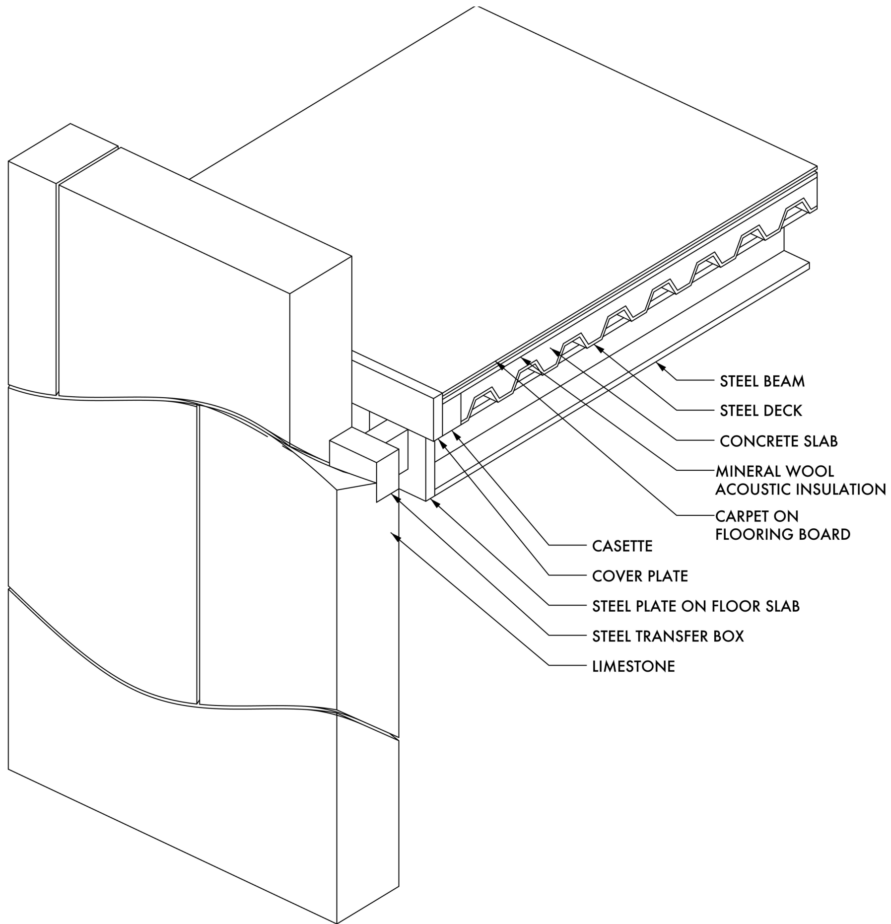
1 Slab Connection / Typical Axonometric Detail 1:20
